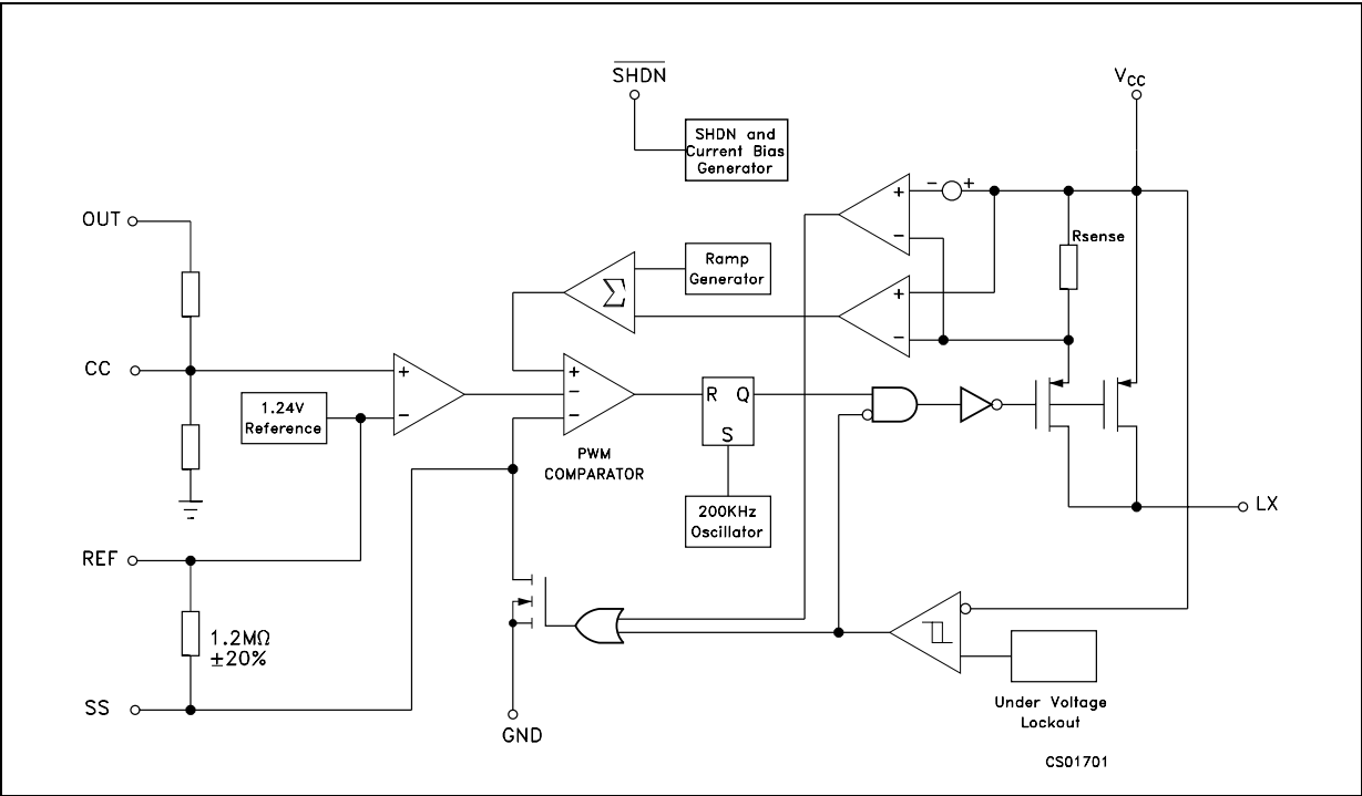
Figure 1. Schematic diagram
