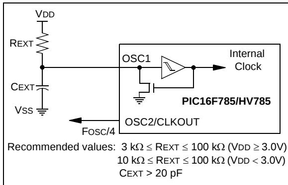
FIGURE 3-5: RC MODE
