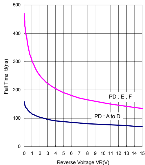
Fall Time vs. Reverse Voltage ( T_a=25^\circ\text{C} )
