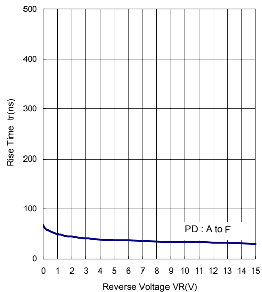
Rise Time vs. Reverse Voltage ( T_a=25^\circ\text{C} )
