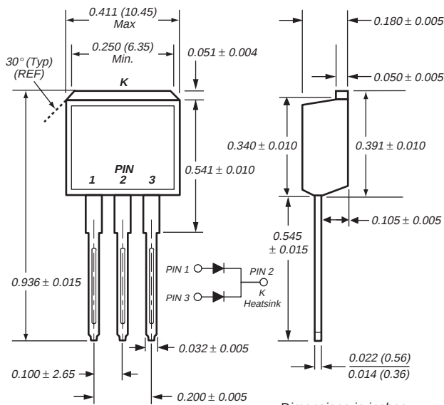
TO-262AA (MBRB3045CT-1, MBRB3045CT-1)
