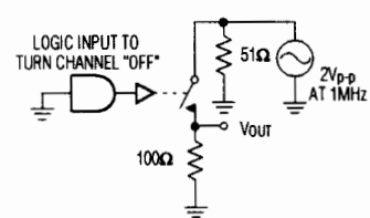
Figure 3. Off-Isolation Rejection Ratio
