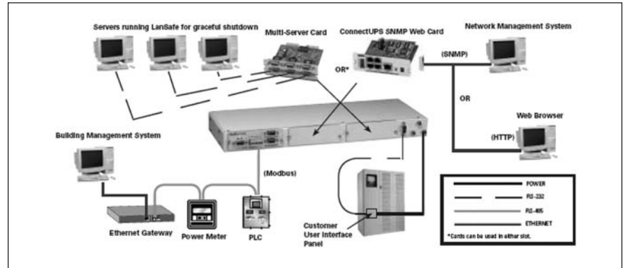
Figure 33.4-2. Typical Configuration
