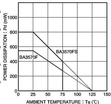
Fig.20 Thermal derating curve
