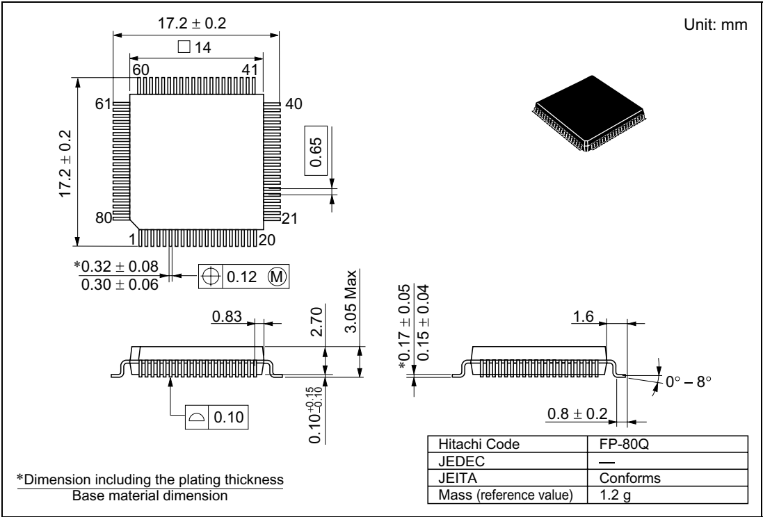
Figure D-1 FP-80Q Package Dimensions
