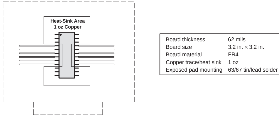
Figure 24. PWB Layout (Including Copper Heatsink Area) for Thermally Enhanced PWP Package
