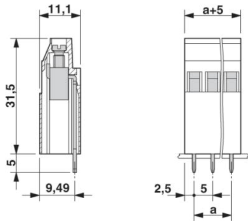
Dimensioned drawing
