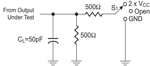
Load Circuit
