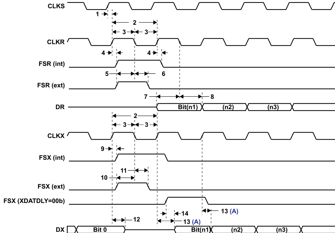
Figure 6-34. McBSP Timing
