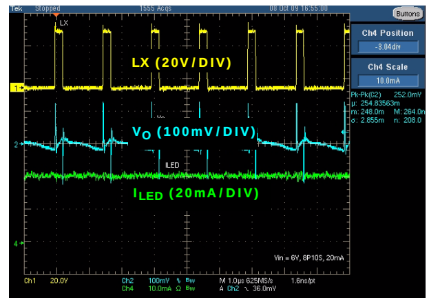
FIGURE 14. V_{\text{OUT}} RIPPLE VOLTAGE
