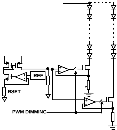
FIGURE 24. SIMPLIFIED CURRENT SOURCE CIRCUIT
