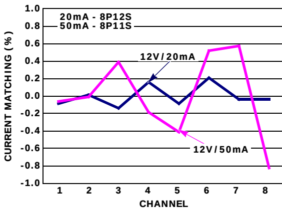
FIGURE 7. CHANNEL-TO-CHANNEL CURRENT MATCHING EXAMPLE
