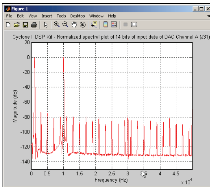
Figure 2–11. Normalized Spectral Plot of 14-Bit DAC Channel A Input Data
