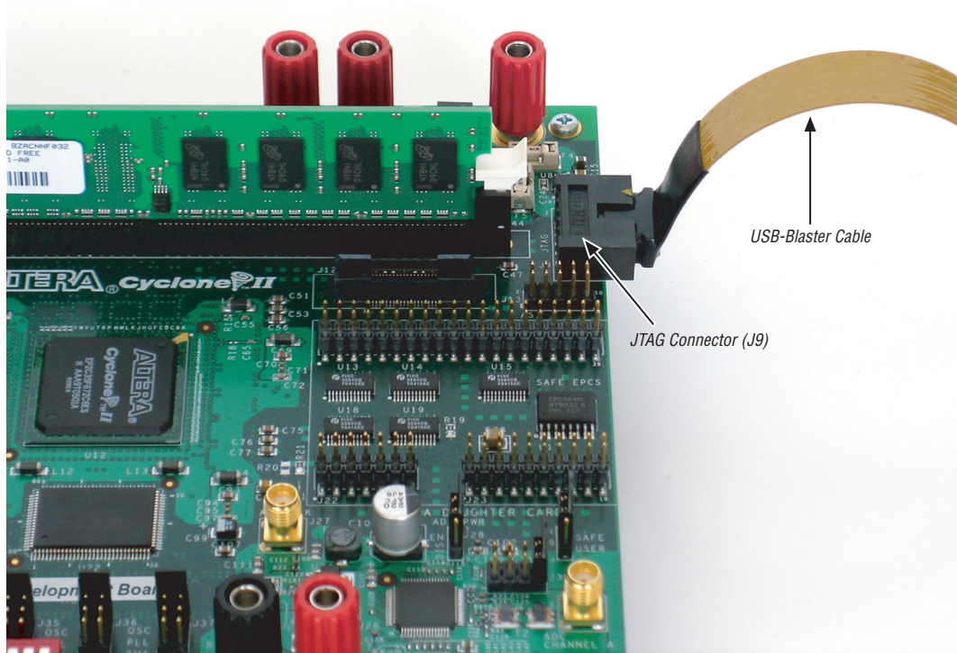
Figure 2–3. Connecting the USB-Blaster Download Cable to J9
