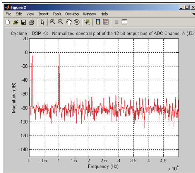
Figure 2–12. Normalized Spectral Plot of 12-bit ADC Channel A Output Data
