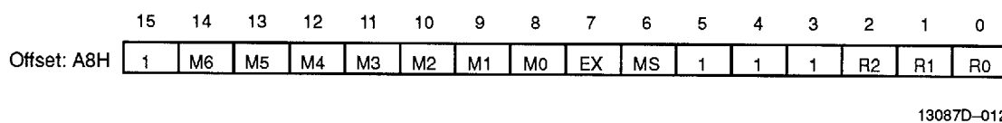
Figure 11. MPSC Register
