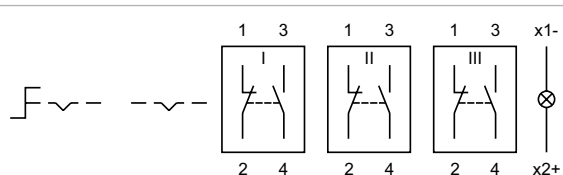
Wiring diagram 27
