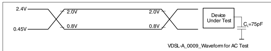
Figure 54 Input and Output Waveform for AC Tests
