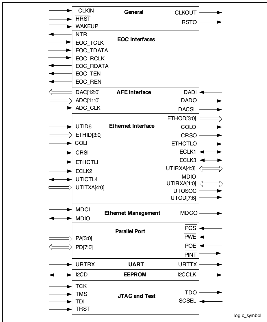
Figure 2 Logic Symbol
