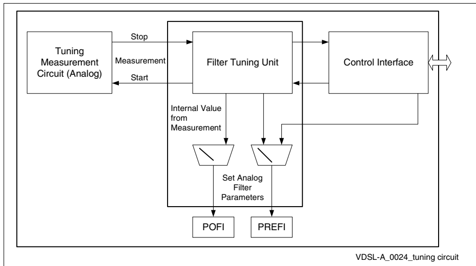
Figure 10 Filter Tuning Unit Functional Block Diagram
