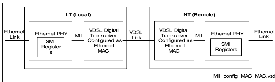
Figure 20 MAC-MAC Scenario
