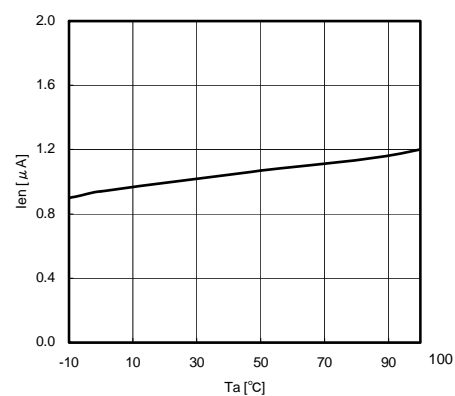
Fig.10 T_a - I_{EN} ( V_{CC}=16\text{V} , V_{EN}=3\text{V} )
