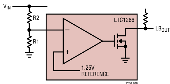
Figure 6. Low-Battery Comparator
