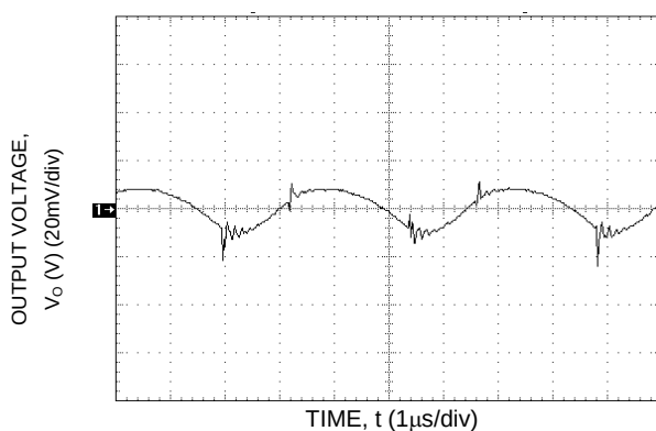
Figure 38. Typical Output Ripple and Noise.
