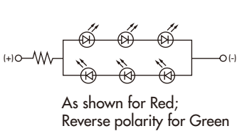
AT621 Bicolor LED 12 & 24-volt 6-element with Resistor
