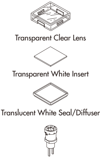
Bicolor LED AT621
