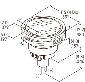
AT3011 Round
