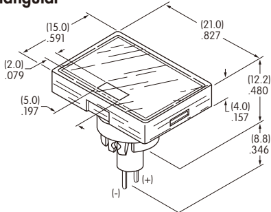
AT3012 Rectangular
