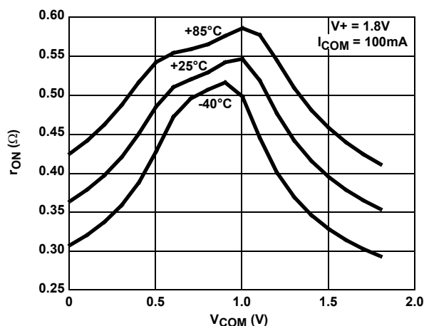
FIGURE 16. ON-RESISTANCE vs SWITCH VOLTAGE
