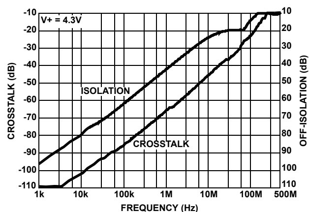
FIGURE 23. CROSSTALK AND OFF-ISOLATION
