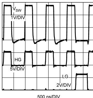
Figure 18. Output Pre-Bias Mode Waveforms
