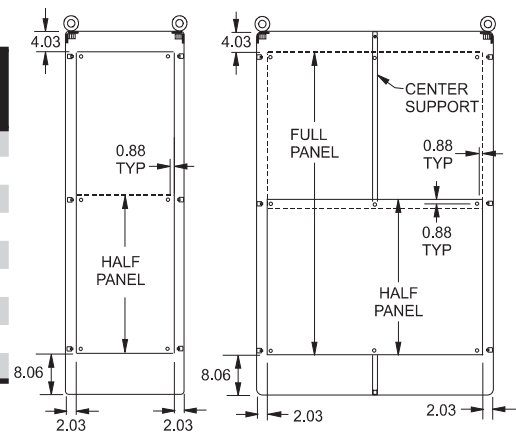
Front View Single Door
