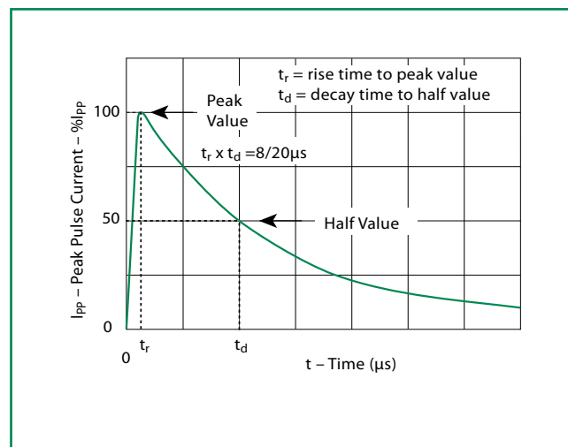
Figure 8 - Pulse Waveform
