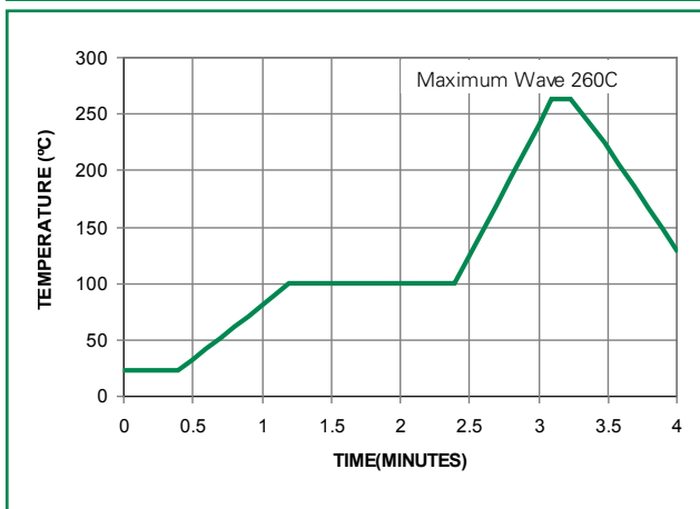
Figure 2 - Lead-free Profile
