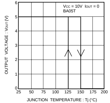
Fig. 8 Thermal cutoff circuit characteristics
