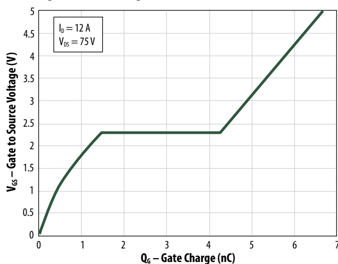
Figure 6: Gate Charge
