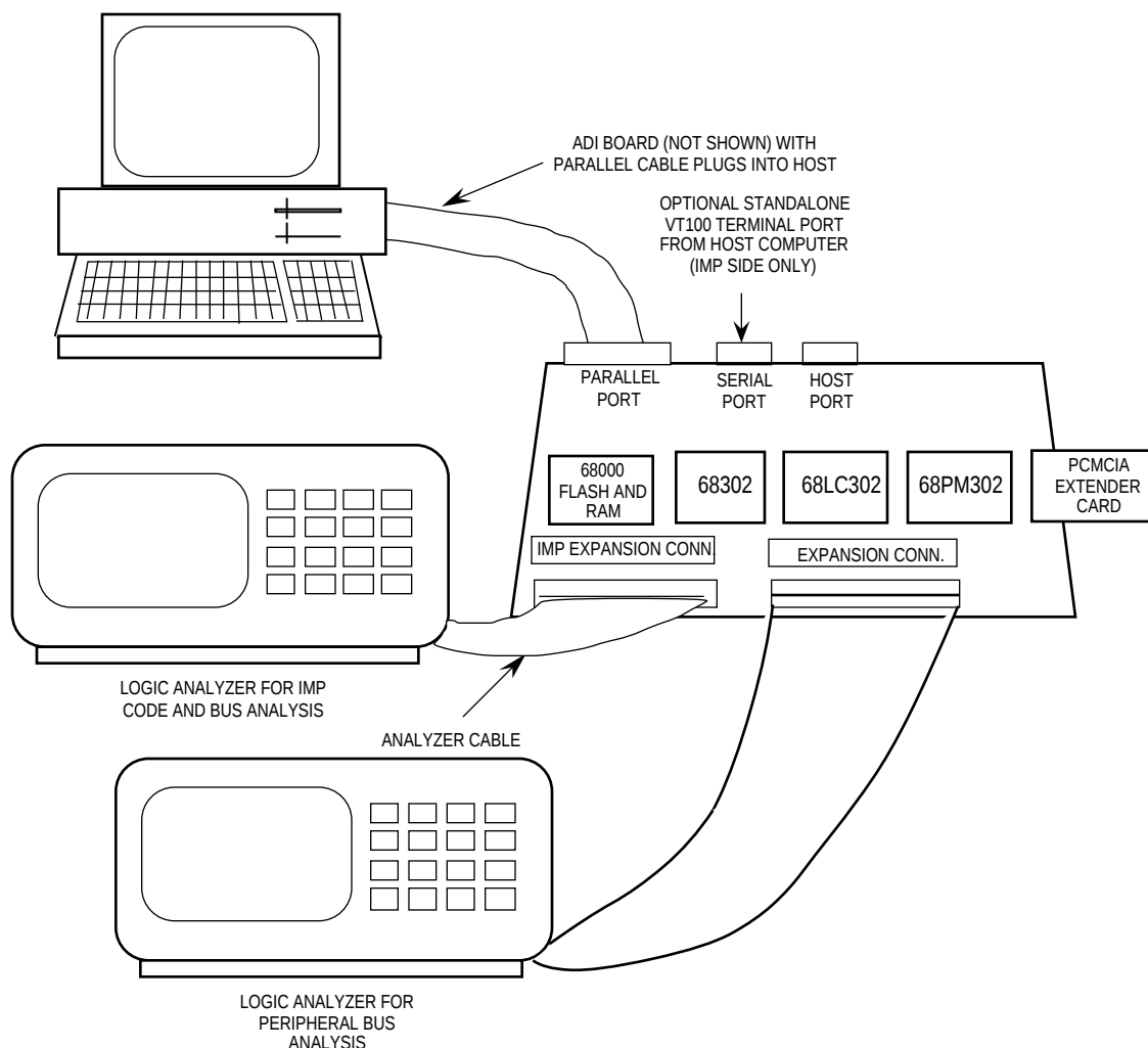
Figure 1. MC68302FADS
