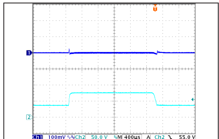
Figure 6: Output voltage response to step-change in input voltage (1000 V/ms). Load cap: 100 μF, electrolytic output capacitance. Ch 1: V out (100 mV/div), Ch 2: V in (50 V/div).
