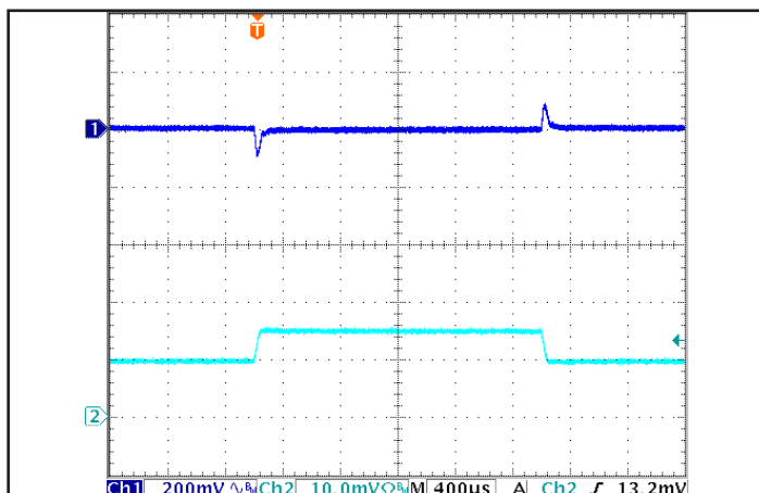
Figure 5: Output voltage response to step-change in load current (50 % -75 % -50 % of I out (max); dI/dt = 0.2 A/μs). Load cap: 100 μF electrolytic capacitor. Ch 1: V out (200mV/div), Ch 2: I out (10 A/div).
