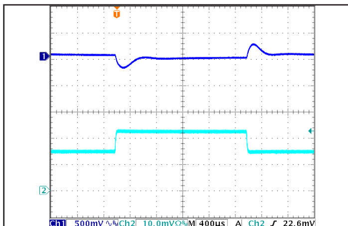
Figure 5: Output voltage response to step-change in load current (50% -75% -50% of I out (max); dI/dt = 0.1 A/μs). Load cap: 100 μF electrolytic capacitor. Ch 1: V out (500 mV/div), Ch 2: I out (1 A/div)
