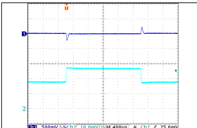
Figure 5: Output voltage response to step-change in load current (50% -75% -50% of I out (max); dI/dt = 0.1 A/μs). Load cap: 100 μF electrolytic capacitor. Ch 1: V out (500 mV/div), Ch 2: I out (2 A/div)
