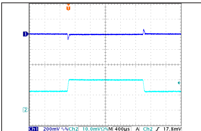
Figure 5: Output voltage response to step-change in load current (50 % -75 % -50 % of I out (max); dI/dt = 0.1 A/μs). Load cap: 100 μF electrolytic capacitor. Ch 1: V out (200 mV/div), Ch 2: I out (10 A/div).
