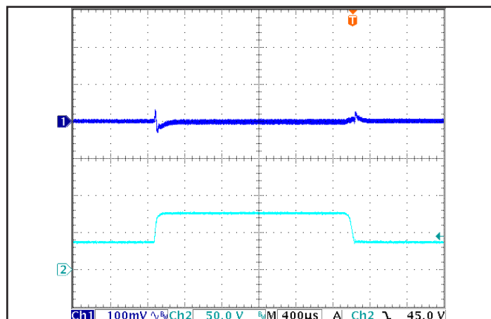
Figure 6: Output voltage response to step-change in input voltage (nominal to maximum, 1000 V/ms). Load cap: 100 μF electrolytic capacitor. Ch 1: V out (100mV/div), Ch 2: V in (50V/div).
