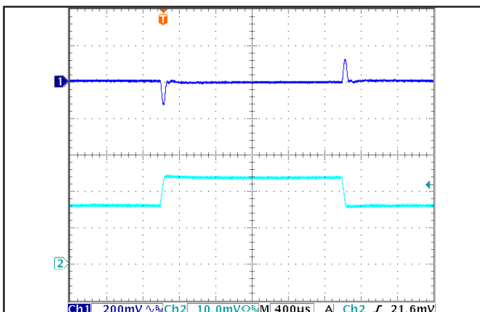
Figure 5: Output voltage response to step-change in load current (50 % -75 % -50 % of Iout(max); dI/dt = 0.1 A/μs). Load cap: 100 μF electrolytic capacitor. Ch 1: Vout (200 mV/div), Ch 2: Iout (5 A/div).
