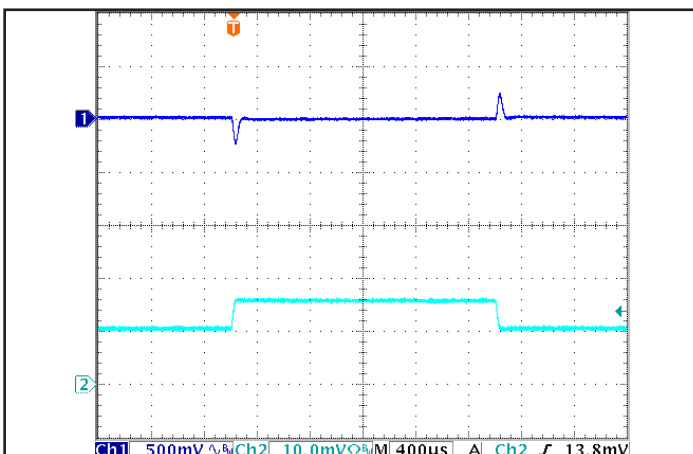
Figure 5: Output voltage response to step-change in load current (50 % -75 % -50 % of I out (max); dI/dt = 0.1 A/μs). Load cap: 100 μF electrolytic capacitor. Ch 1: V out (500 mV/div), Ch 2: I out (5 A/div)
