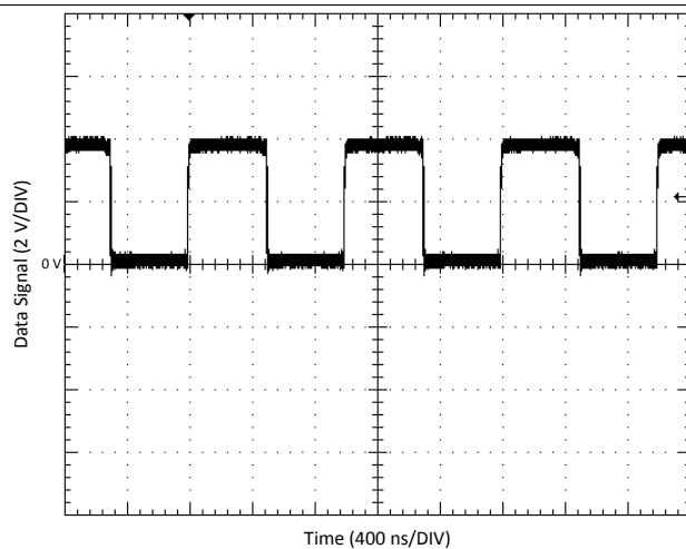
Figure 15. Receiver Single-Ended Output Signal
