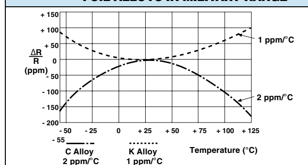
FIGURE 1 - FOIL RESISTOR TCR COMPARISON OF FOIL ALLOYS IN MILITARY RANGE
