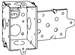
804 S S bracket recessed 5/8"
