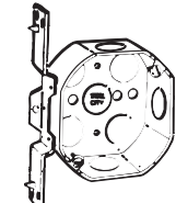
54151 V 1/2 V bracket recessed 1/2"
