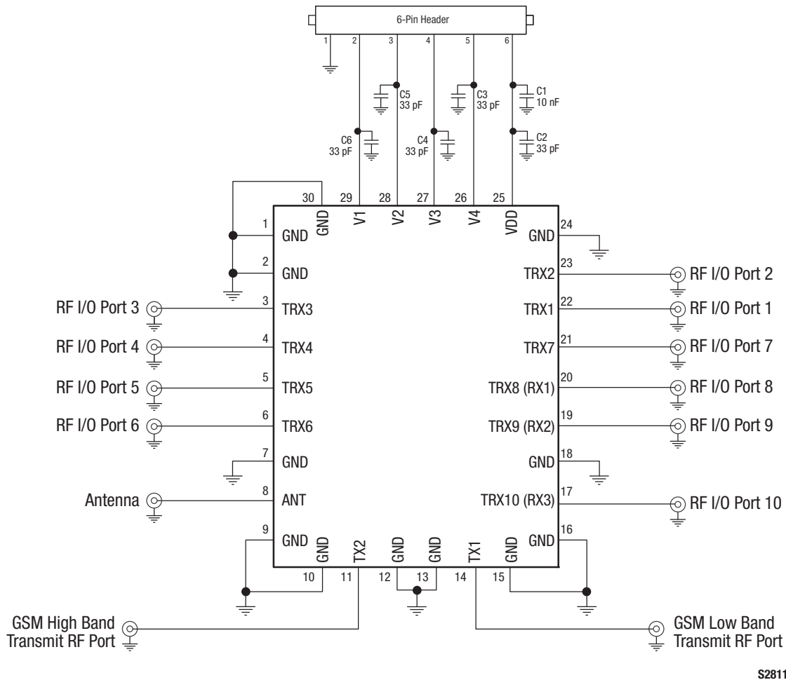
Figure 4. SKY13412-487LF Evaluation Board Schematic
