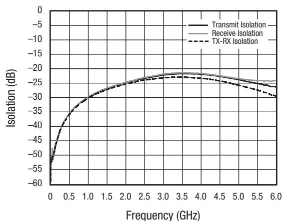
Figure 4. Typical Isolation
