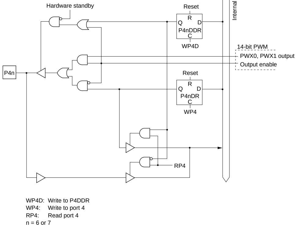
Figure C.12 Port 4 Block Diagram (Pins P46, P47)
