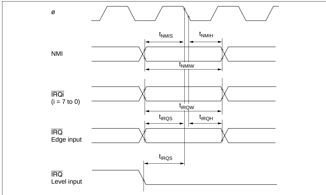
Figure 26.9 Interrupt Input Timing
