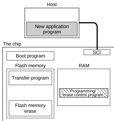
Figure 22.5 User Program Mode (Example)
