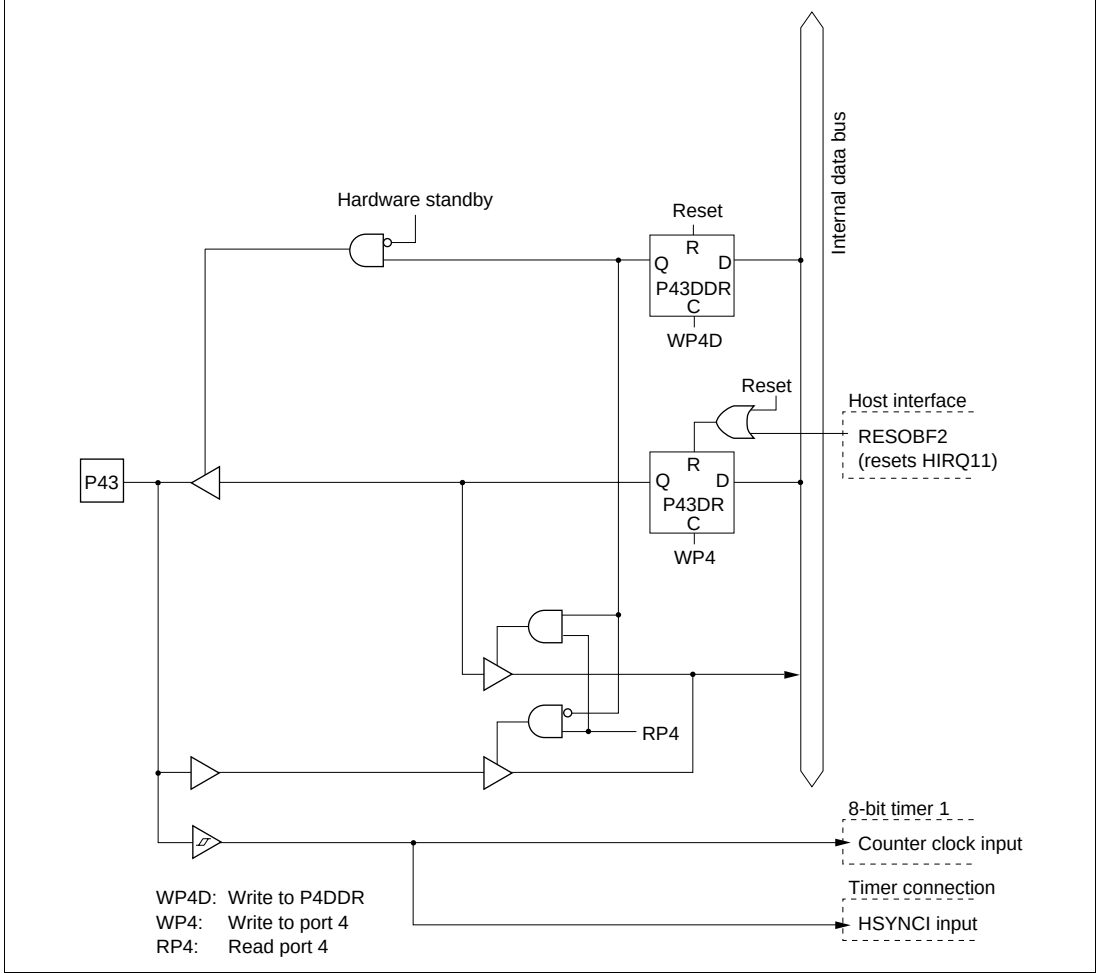
Figure C.9 Port 4 Block Diagram (Pin P43)
