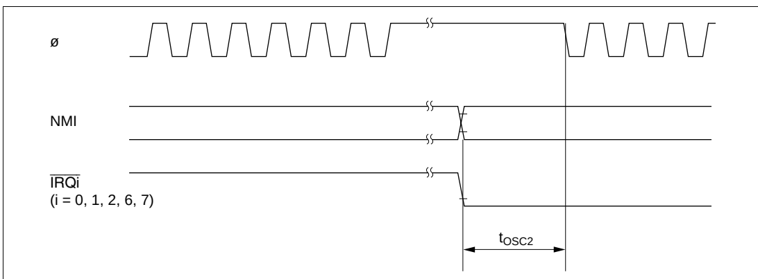
Figure 26.7 Oscillation Setting Timing (Exiting Software Standby Mode)
