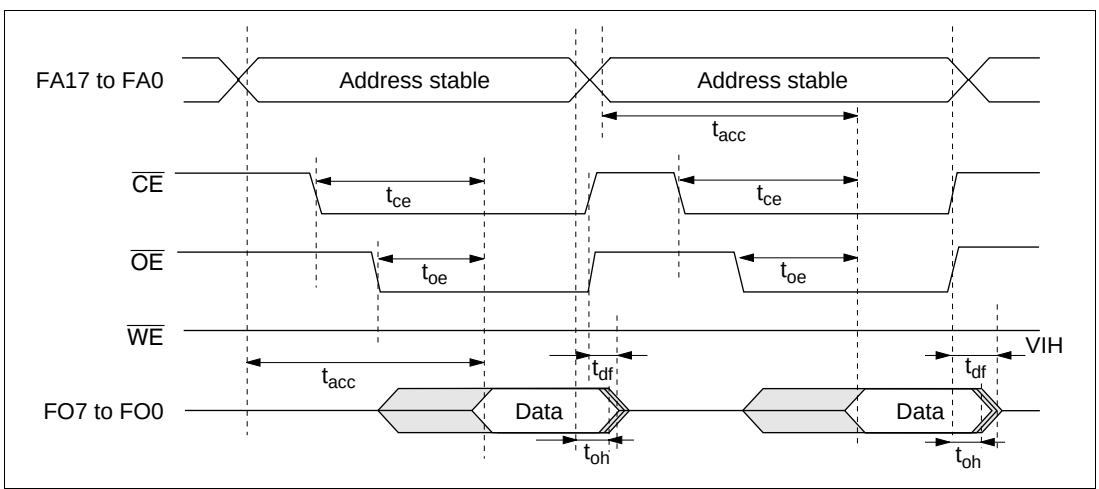
Figure 23.19 Timing Waveforms for \overline{CE}/\overline{OE} Clocked Read
