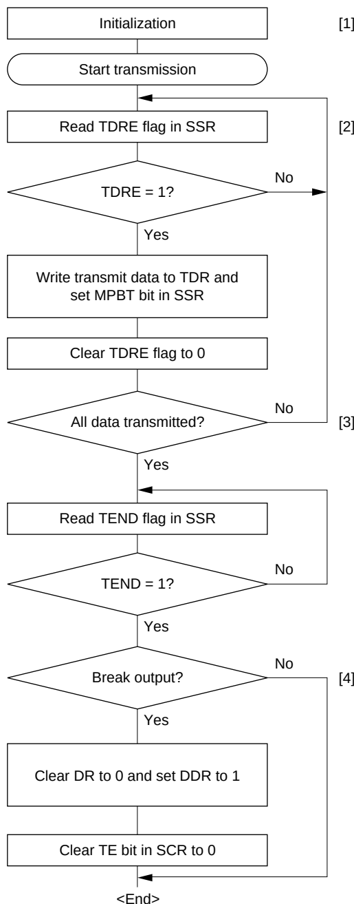
Figure 15.10 Sample Multiprocessor Serial Transmission Flowchart
