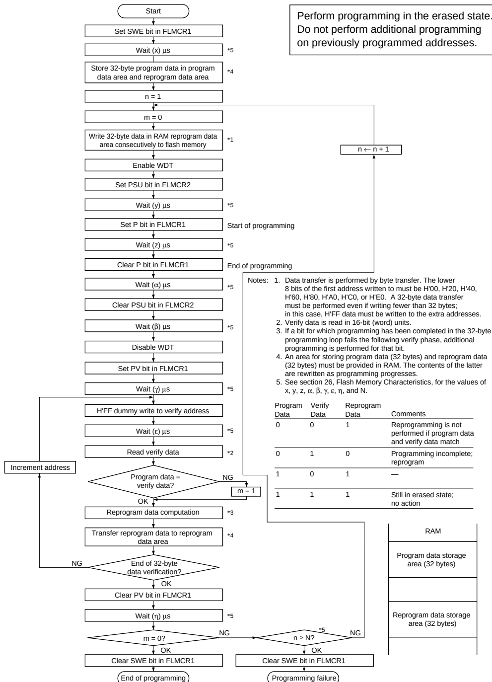
Figure 22.12 Program/Program-Verify Flowchart
