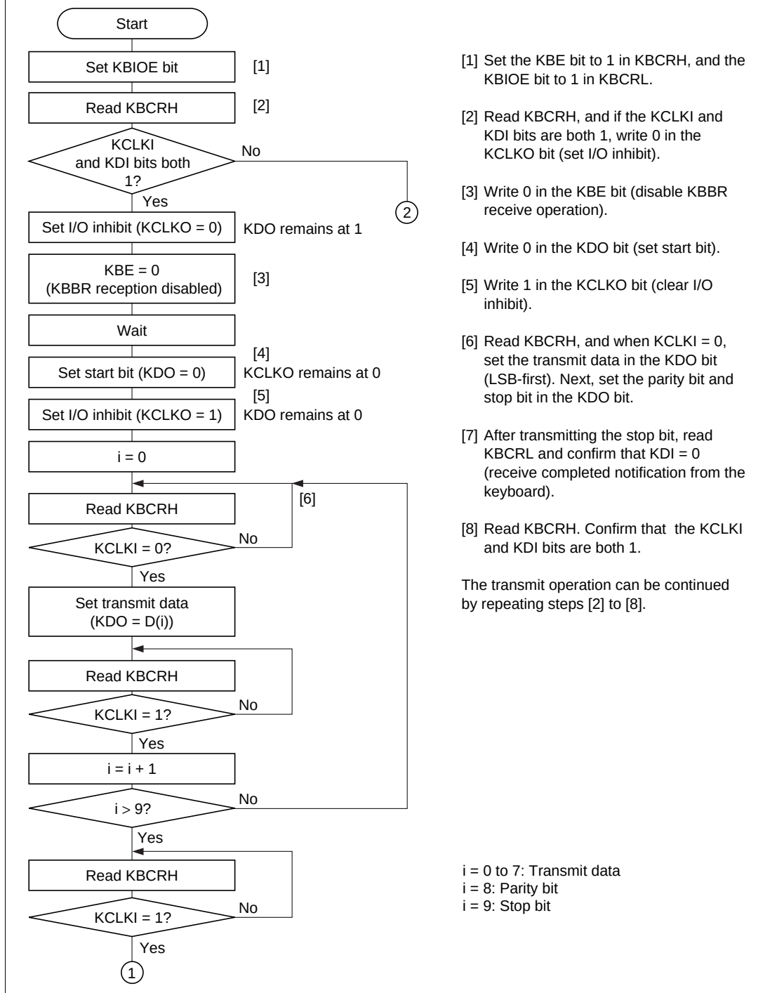
Figure 17.5 Sample Transmit Processing Flowchart
