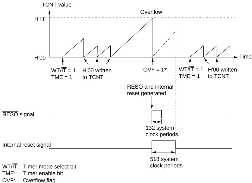
Figure 14.3 Operation in Watchdog Timer Mode ( \text{RST}/\overline{\text{NMI}} = 1 )
