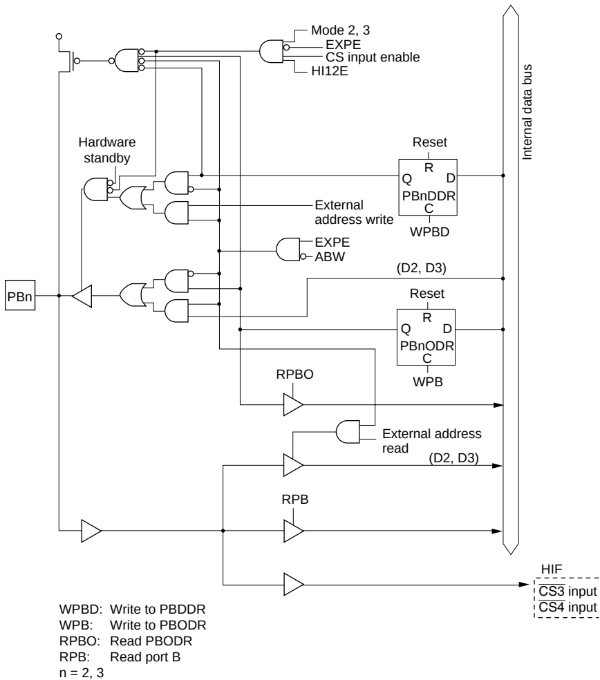
Figure C.38 Port B Block Diagram (Pins PB2 and PB3)
