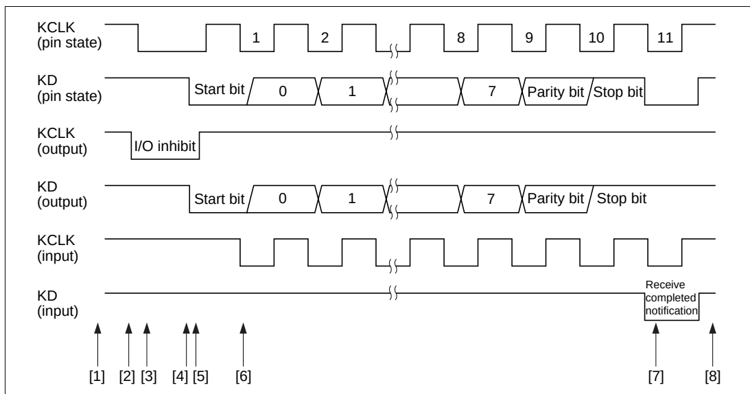
Figure 17.6 Transmit Timing
