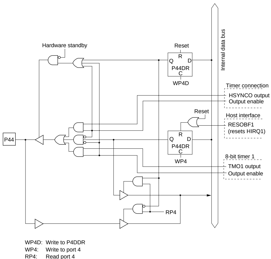
Figure C.10 Port 4 Block Diagram (Pin P44)
