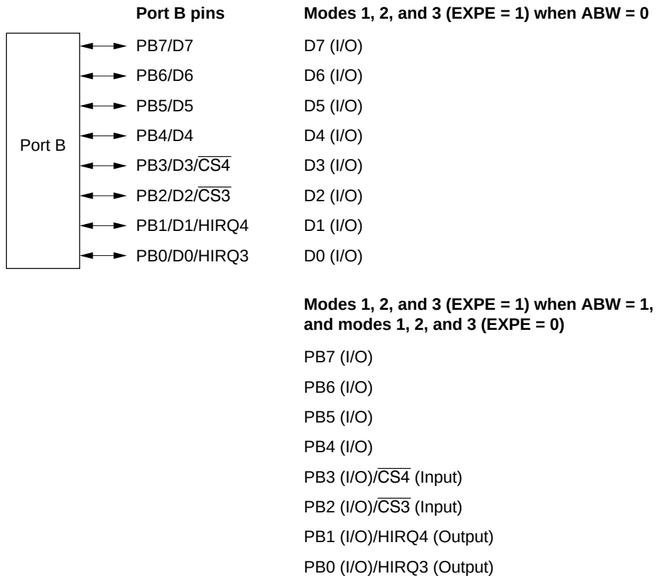
Figure 8.19 Port B Pin Functions
