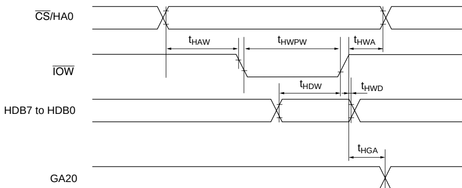
Figure 26.26 Host Interface Timing
