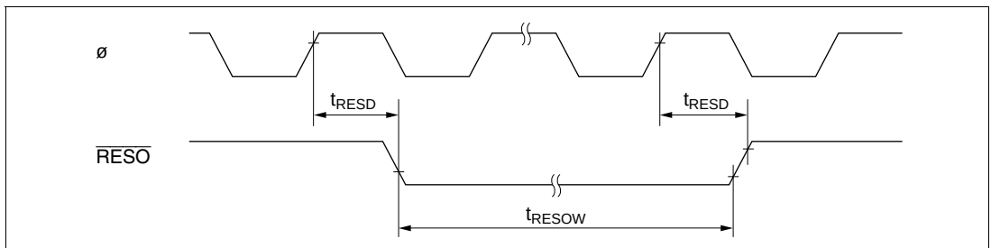
Figure 26.25 WDT Output Timing ( \overline{RESO} )
