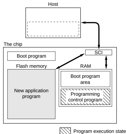
Figure 23.4 Boot Mode
