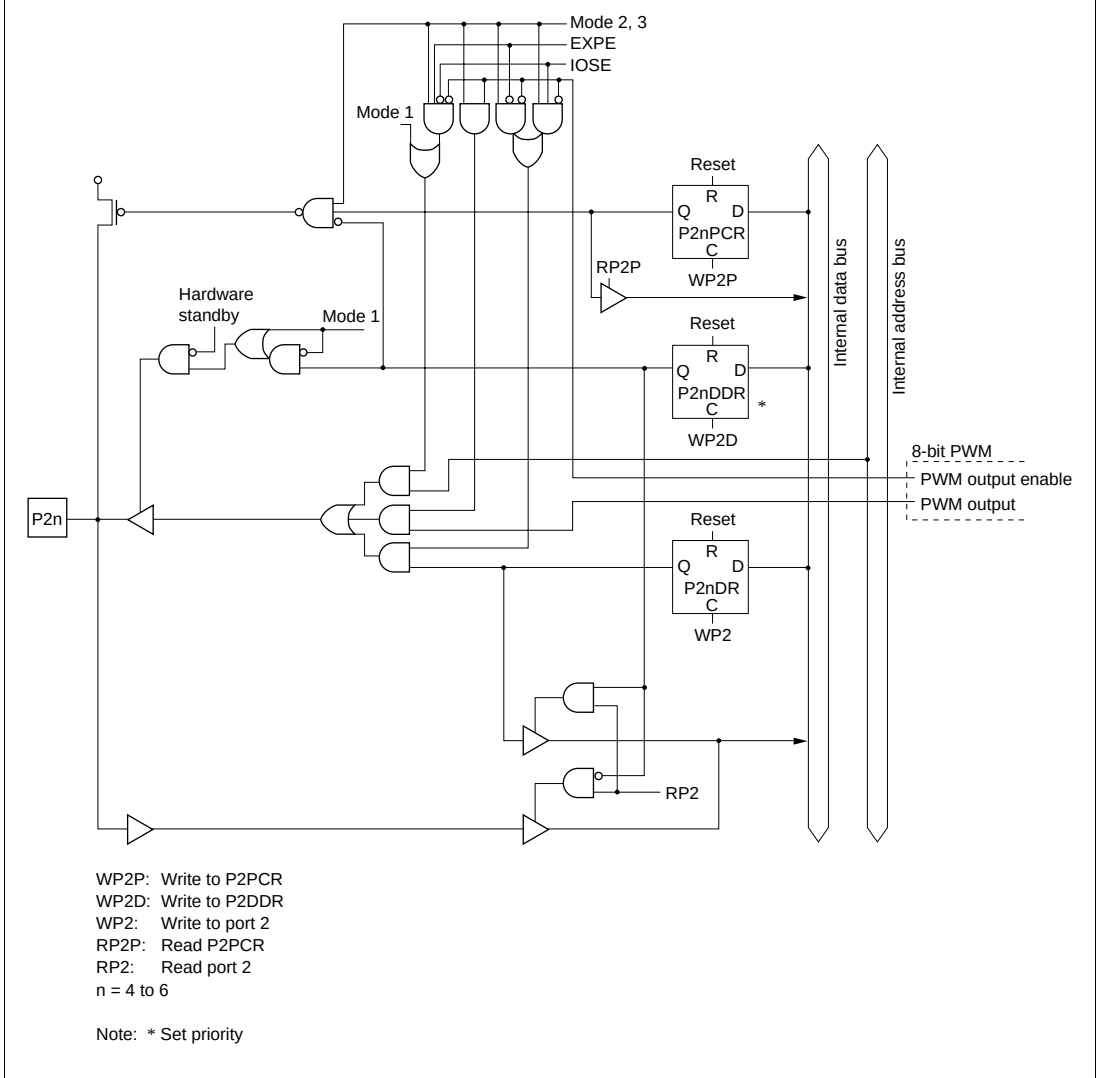
Figure C.3 Port 2 Block Diagram (Pins P24 to P26)
