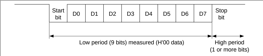
Figure 22.9 RxD1 Input Signal when Using Automatic SCI Bit Rate Adjustment
