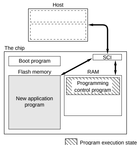
Figure 22.4 Boot Mode
