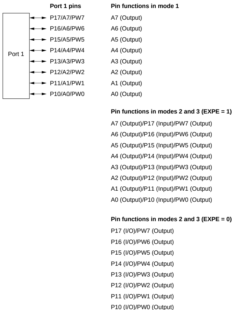
Figure 8.1 Port 1 Pin Functions
