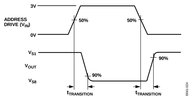
Figure 24. Switching Time of Multiplexer, t_{TRANSITION}
