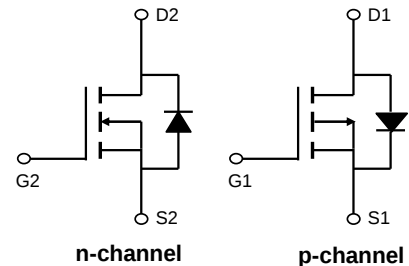
n-channel
