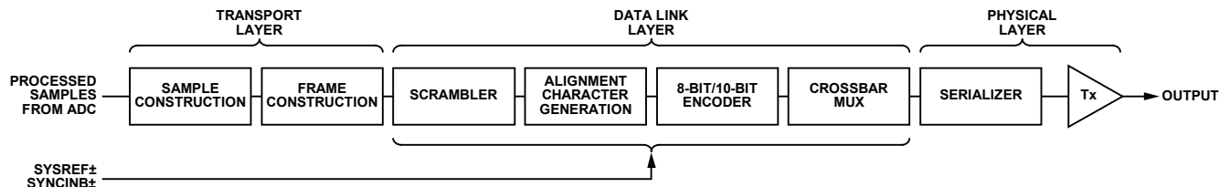
Figure 120. Data Flow
