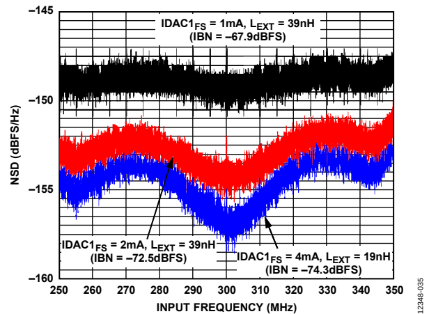
Figure 81. NSD vs. IDAC1_{FS} Setting with Decimate by 16, I/Q Output (IF = 300 MHz, BW = 100 MHz, F_{ADC} = 3.2 GHz)
