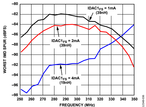
Figure 82. Swept Dual-Tone IMD vs. IDAC1_{FS} Setting with Decimate by 16, I/Q Output, Dual Tones Set to -8 dBFS (IF = 300 MHz, BW = 100 MHz, F_{ADC} = 3.2 GHz)
