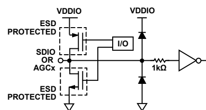
Figure 62. Equivalent SDIO or AGC Input/Output Circuit
