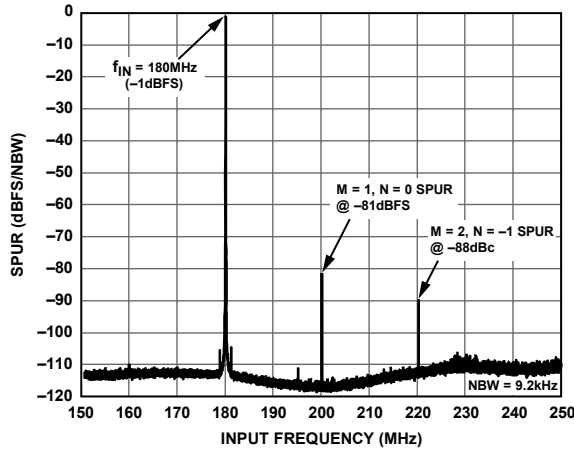
Figure 137. Image Spur for f_{\text{DATA\_IQ}} = 200 MSPS ( \text{DEC\_MODE} = 3 ) Attributed to M = 2, N = -1
