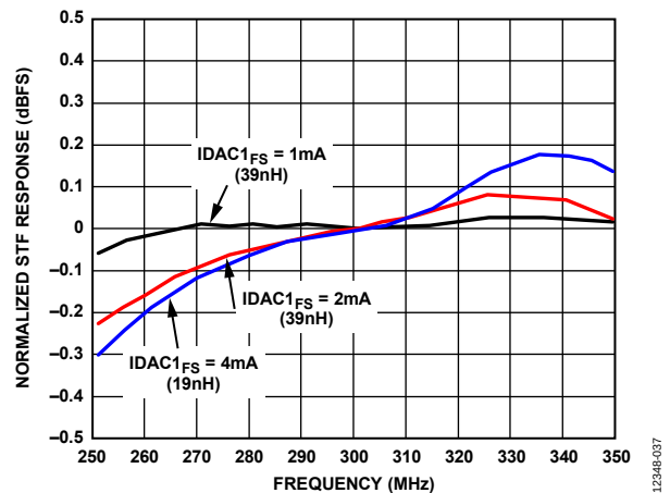
Figure 83. STF vs. IDAC1_{FS} Setting with Decimate by 16, I/Q Output, Dual Tones Set to -8 dBFS (IF = 300 MHz, BW = 100 MHz, F_{ADC} = 3.2 GHz)
