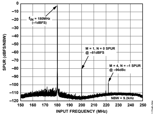
Figure 138. Reduction in Image Spur When f_{\text{DATA\_IQ}} is Reduced to 100 MSPS
