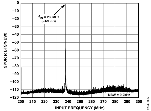
Figure 139. Digital Induced Spurs for an IF That Is Centered Between f_{\text{DATA\_IQ}} and 1.5 \times f_{\text{DATA\_IQ}} with f_{\text{DATA\_IQ}} = 200 MSPS
