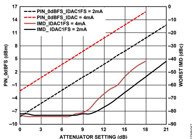
Figure 96. IMD Component Degradation as Two-Tone Centered at an IF of 180 MHz Is Increased 1 dB for Every 1 dB Increase in Attenuator Setting, Such That Two-Tone Level Remains at -8 dBFS
