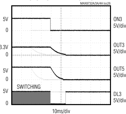
SHUTDOWN WAVEFORMS
