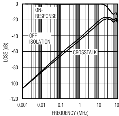
FREQUENCY RESPONSE (µMAX)
