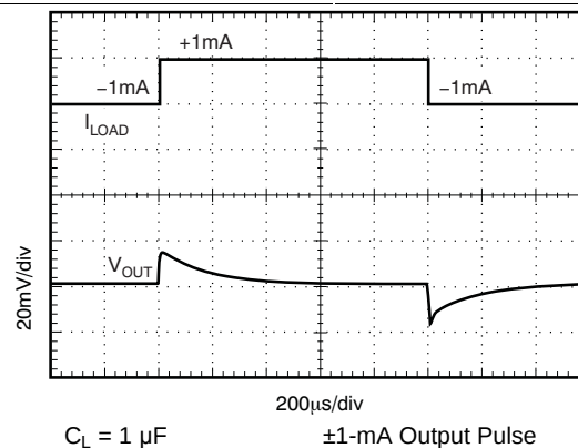
Figure 14. Load Transient
