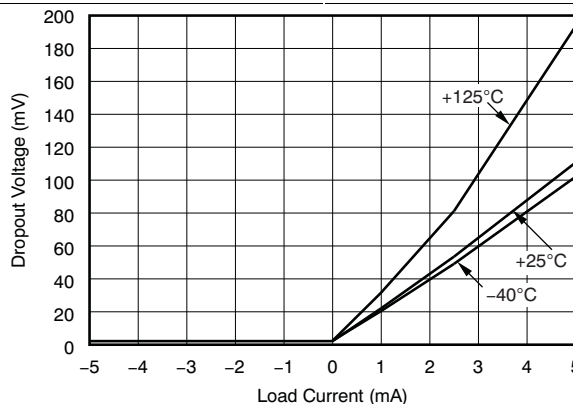
Figure 2. Temperature Drift
