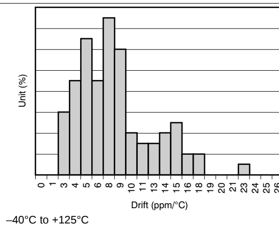
Figure 2. Temperature Drift
