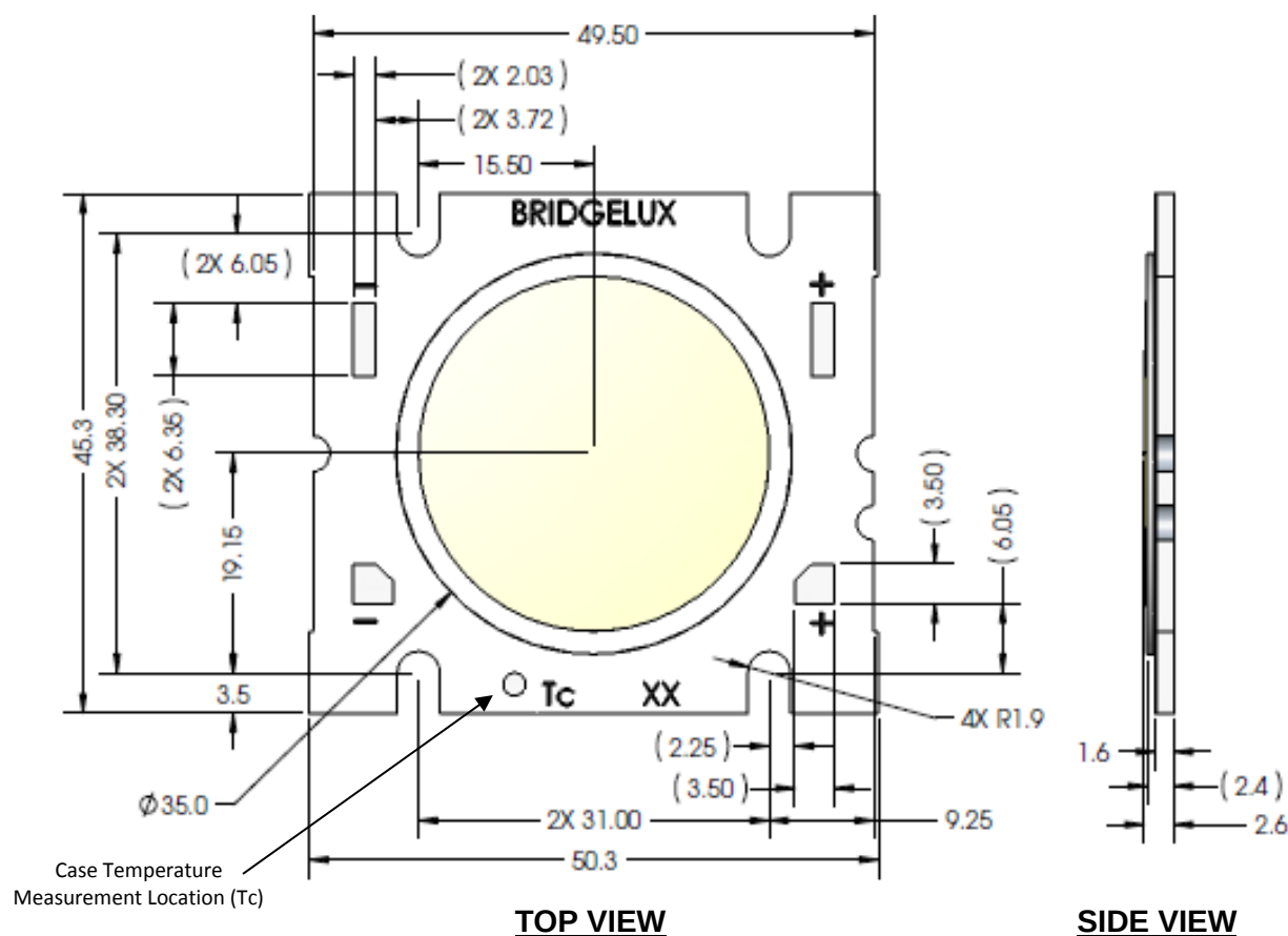
Figure 18: Drawing for RS Part Numbers BXRA-xxH4000-H-03 and BXRA-xxH7000-J-03
