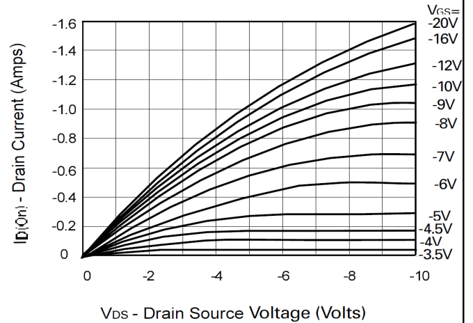
Saturation Characteristics
