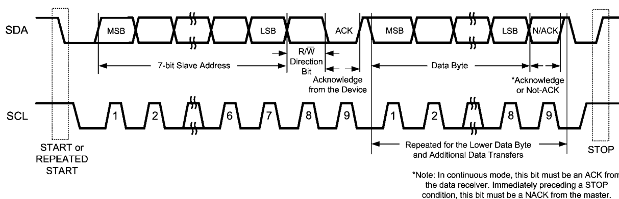
FIGURE 7. Basic Operation.
