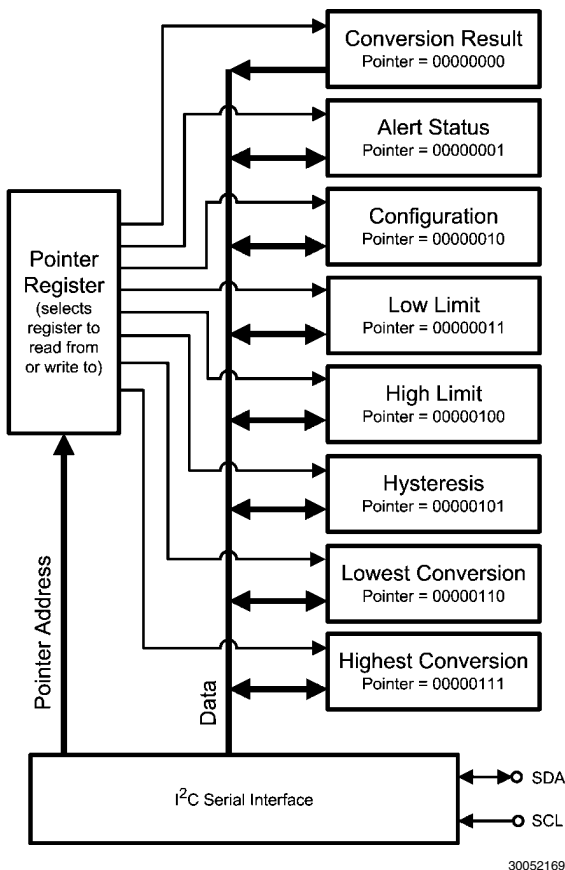
FIGURE 6. Register Structure
