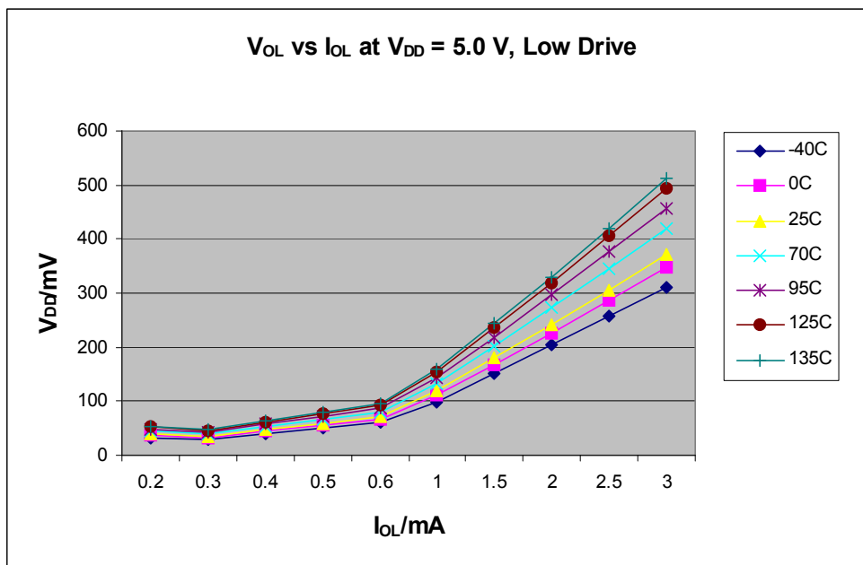
Figure 6. Typical V_{OL} vs. I_{OL} for Low Drive Enabled Pad ( V_{DD} = 5 V)
