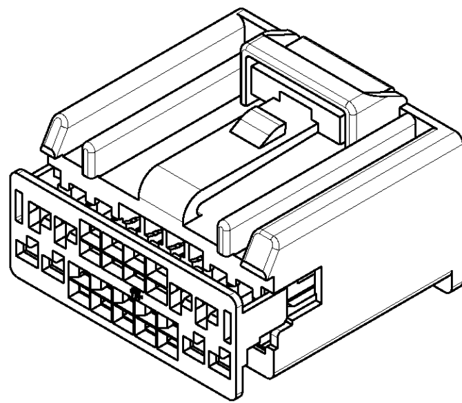
638116-1 KEY A CONFIGURATION SCALE 2:1
