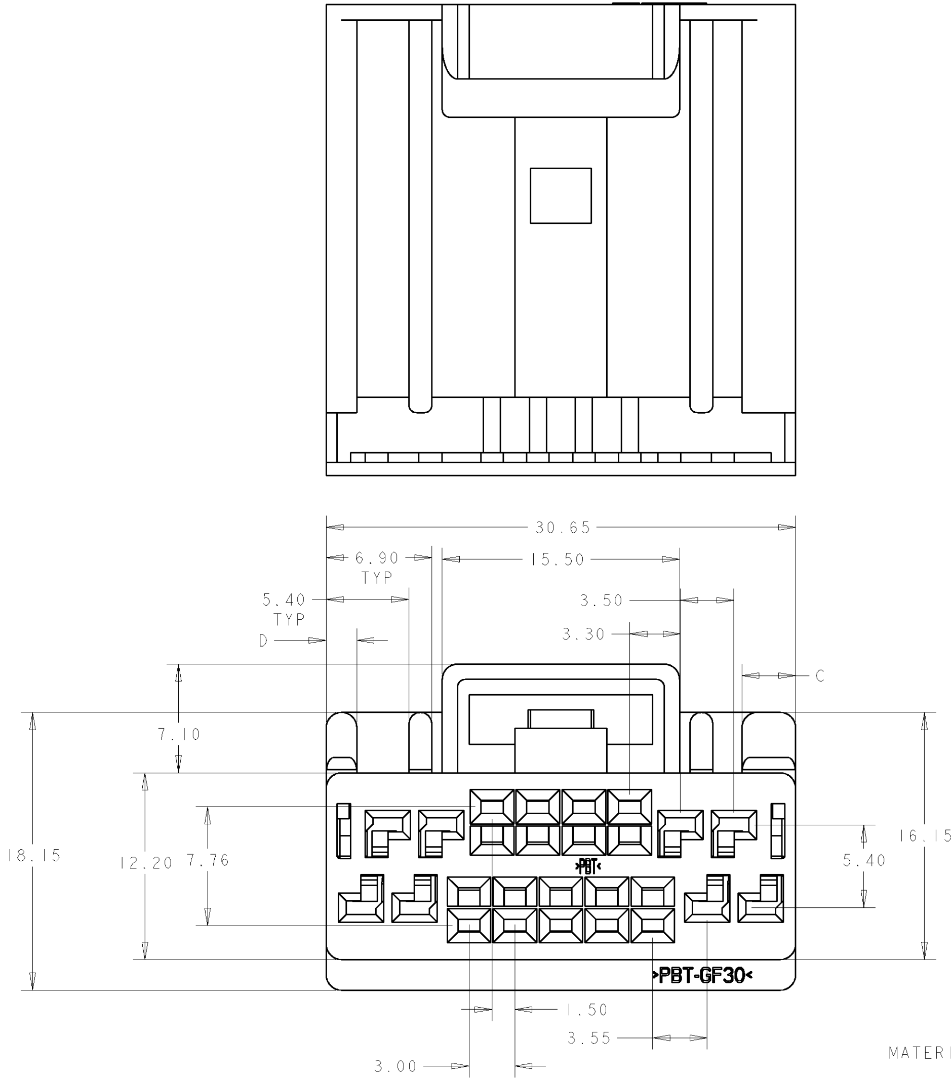
638116-1 SHOWN KEY A CONFIGURATION
