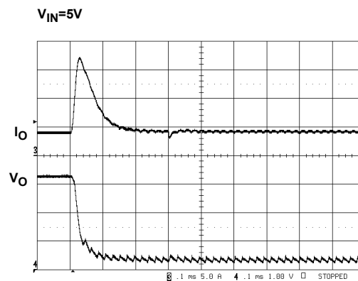
FIGURE 20. SHORT-CIRCUIT PROTECTION
