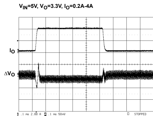
FIGURE 15. TRANSIENT RESPONSE
