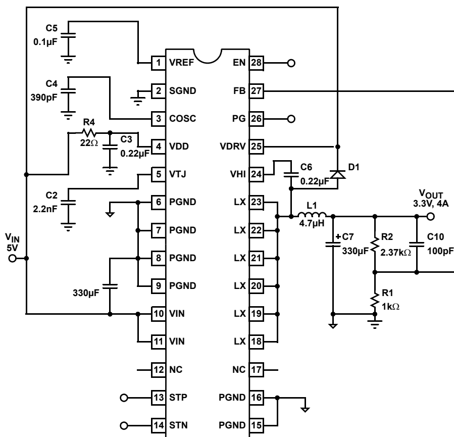
EL7654 (28-PIN HTSSOP) TOP VIEW
