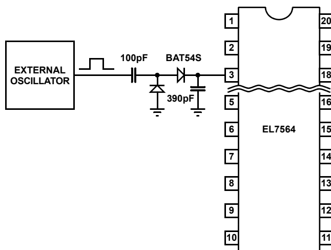
FIGURE 23. OSCILLATOR SYNCHRONIZATION
