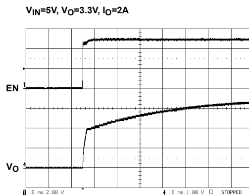
FIGURE 18. RELEASING EN
