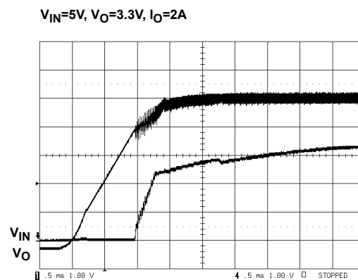
FIGURE 16. POWER-UP
