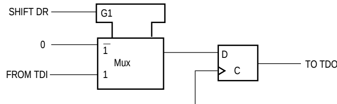
Figure 8-8. Bypass Register
