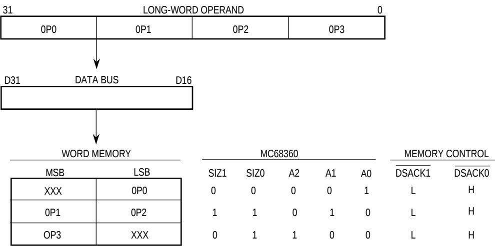
Figure 4-8. Misaligned Long-Word Transfer to Word Port Example
