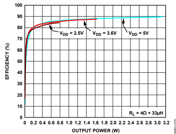
Figure 20. Efficiency vs. Output Power, R_L = 4\Omega + 33\mu\text{H}
