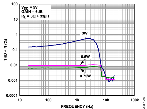
Figure 8. THD + N vs. Frequency, V_{DD} = 5V , R_L = 3\Omega + 33\mu H , Gain = 6 dB
