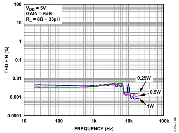
Figure 6. THD + N vs. Frequency, V_{DD} = 5V , R_L = 8\Omega + 33\mu H , Gain = 6 dB
