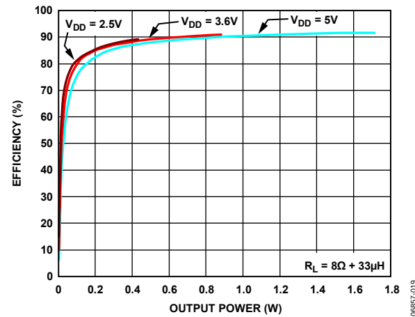
Figure 19. Efficiency vs. Output Power, R_L = 8\Omega + 33\mu\text{H}
