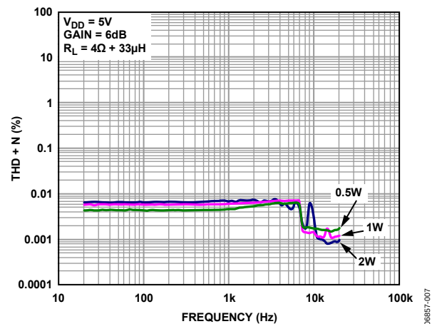
Figure 7. THD + N vs. Frequency, V_{DD} = 5V , R_L = 4\Omega + 33\mu H , Gain = 6 dB
