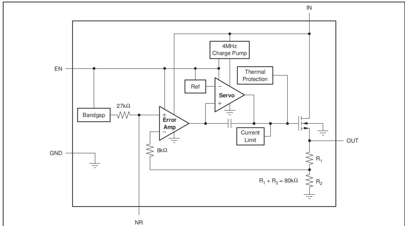
Figure 6-1. Fixed-Voltage Version
